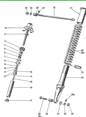
M 125
